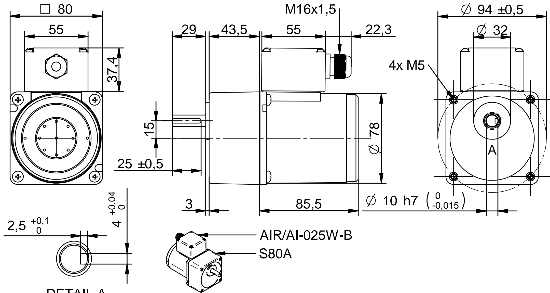
DETAIL A SCALE 1.4:1 Label
